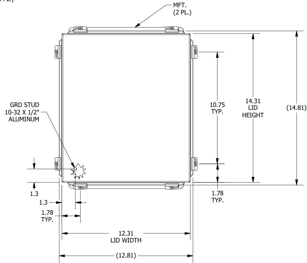
FRONT VIEW
