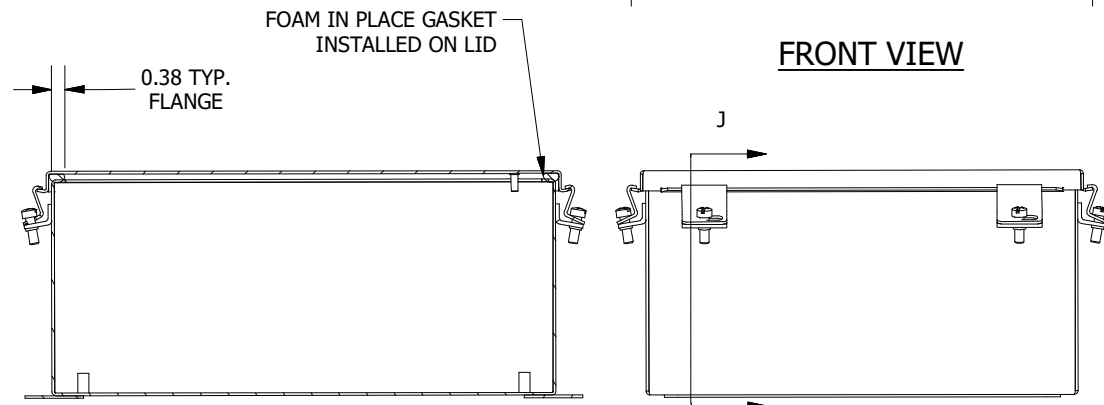
SECTION J-J
