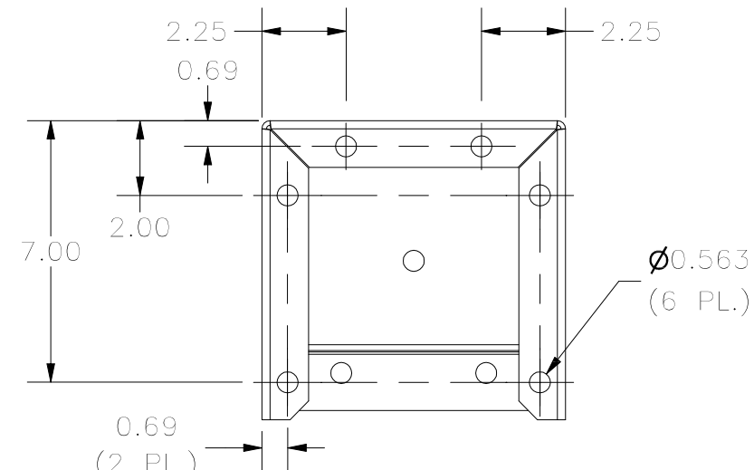
BOTTOM VIEW
