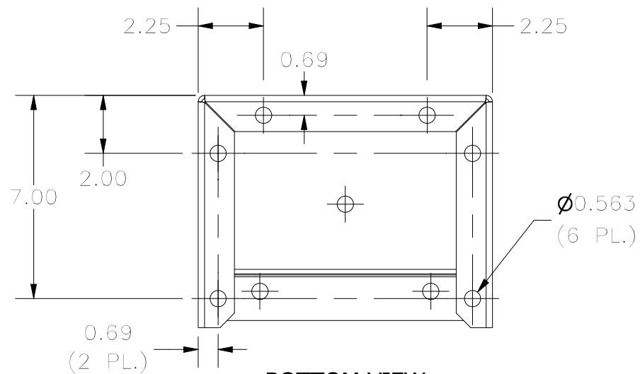
BOTTOM VIEW
