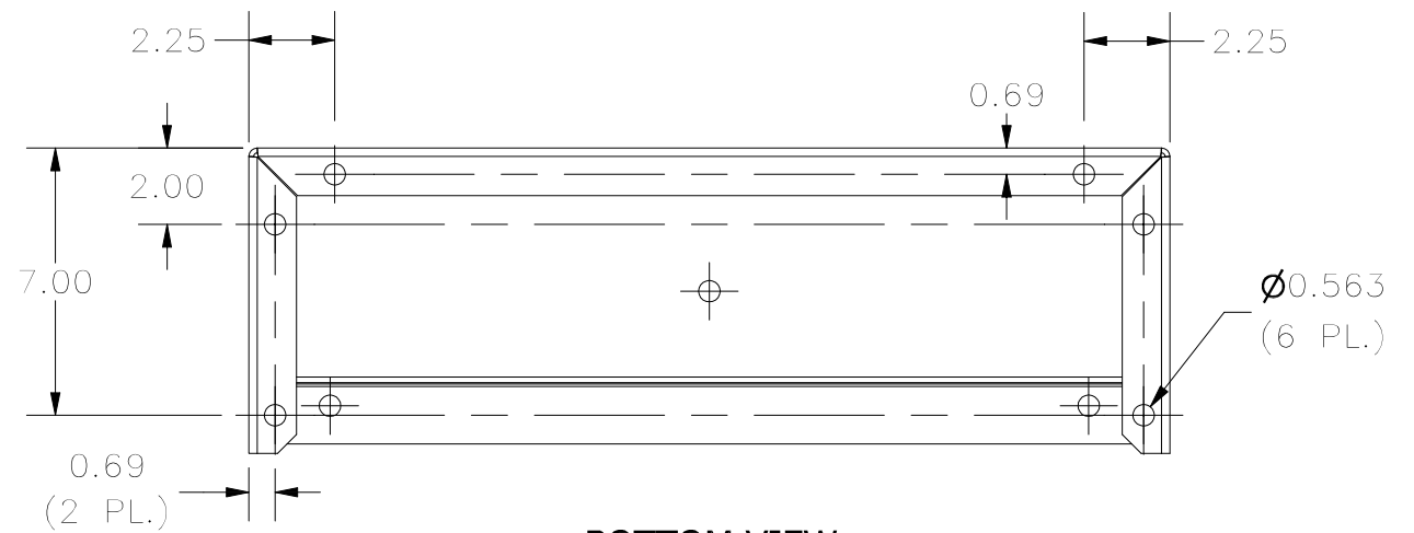
BOTTOM VIEW
