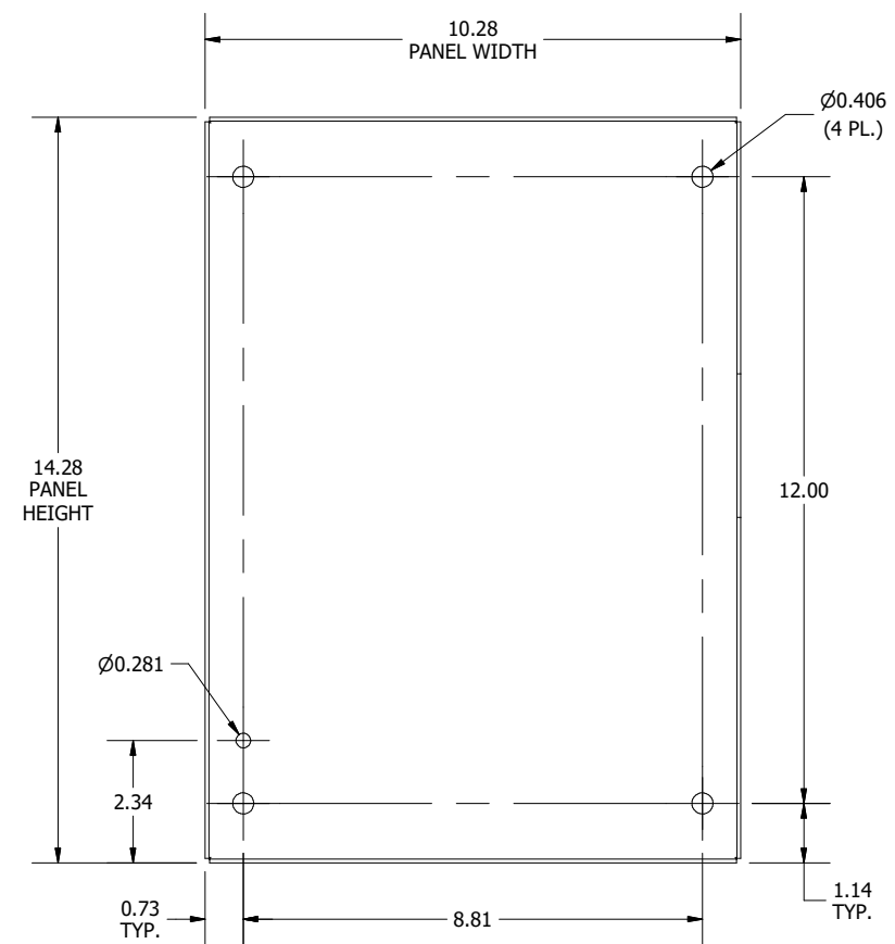
PANEL ONLY FRONT VIEW
