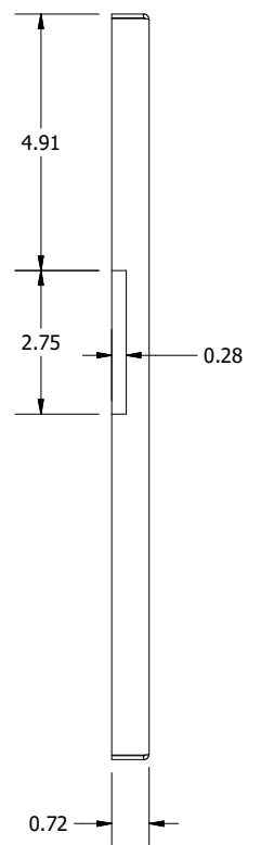
PANEL ONLY RIGHT SIDE VIEW
