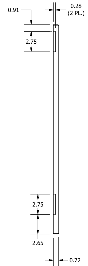
PANEL ONLY RIGHT SIDE VIEW
