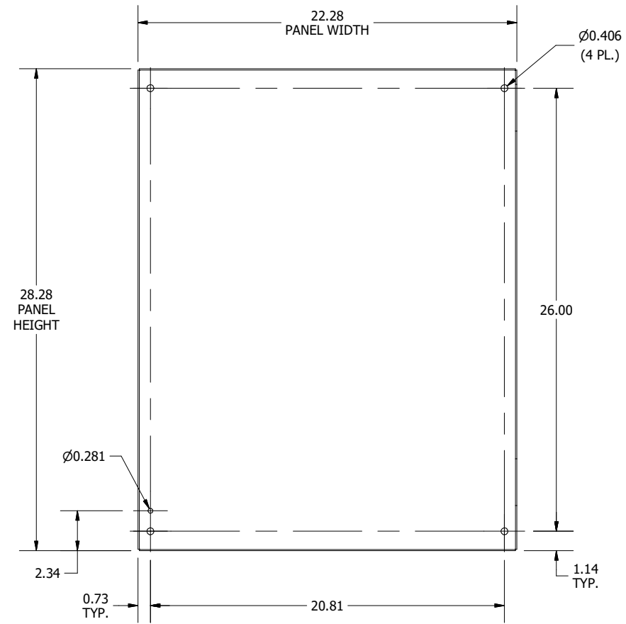
PANEL ONLY FRONT VIEW
