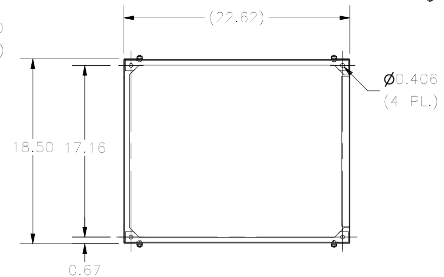
FRONT VIEW (SWING PANEL REMOVED)
