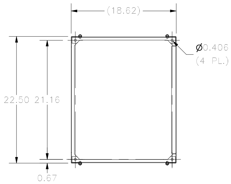
FRONT VIEW (SWING PANEL REMOVED)
