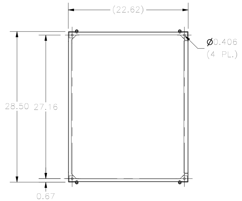
FRONT VIEW (SWING PANEL REMOVED)
