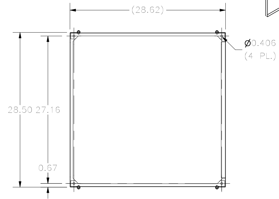
FRONT VIEW (SWING PANEL REMOVED)
