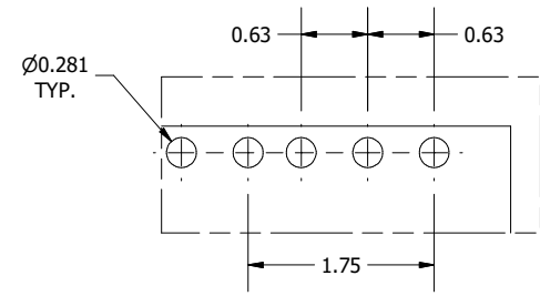
DETAIL A (TYP.) (REPEATING PATTERN FOR STANDARD 19" RACK EQUIPMENT, 12U)
