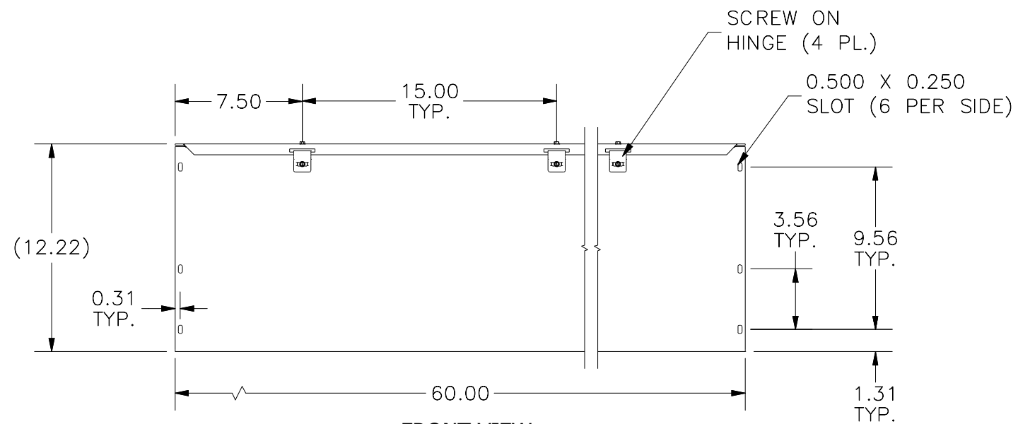
FRONT VIEW
