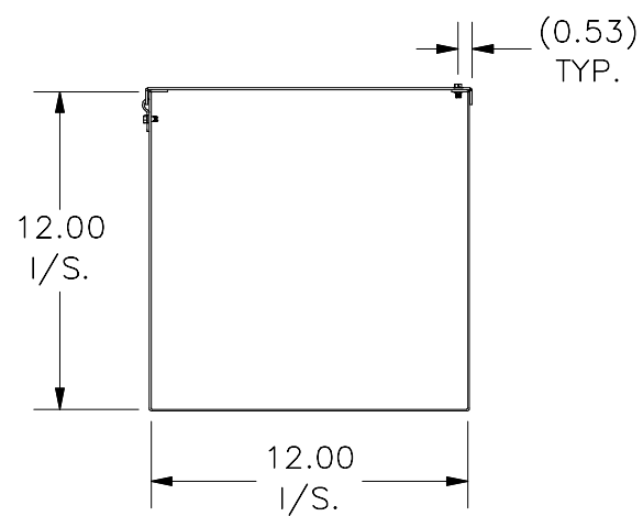
RIGHT VIEW
