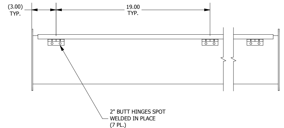
BACK VIEW
