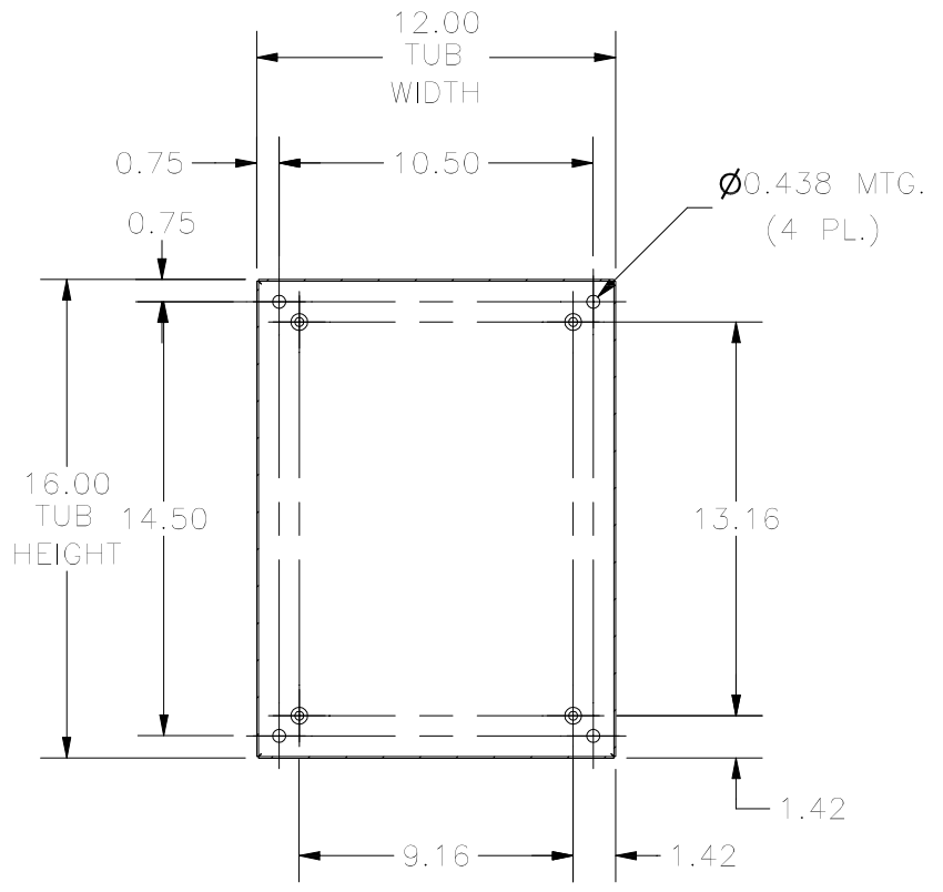
SECTION W-W (INSIDE BACK OF ENCLOSURE)
