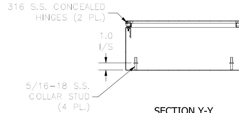
SECTION Y-Y (INSIDE TOP OF ENCLOSURE)
