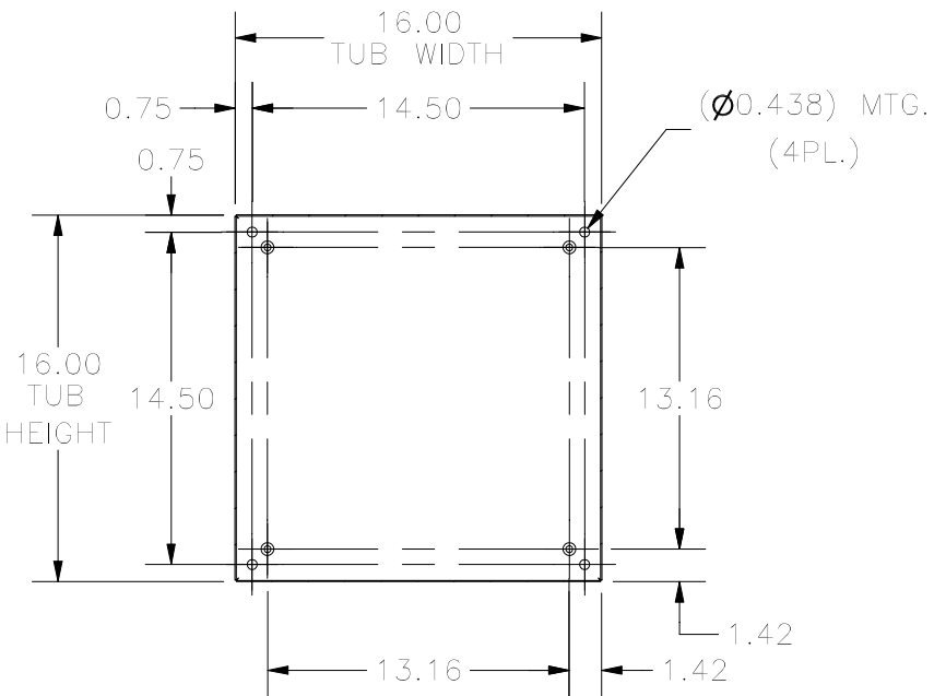
SECTION W-W (INSIDE BACK OF ENCLOSURE)
