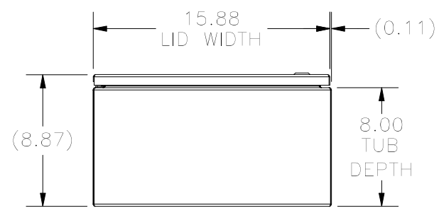
BOTTOM VIEW
