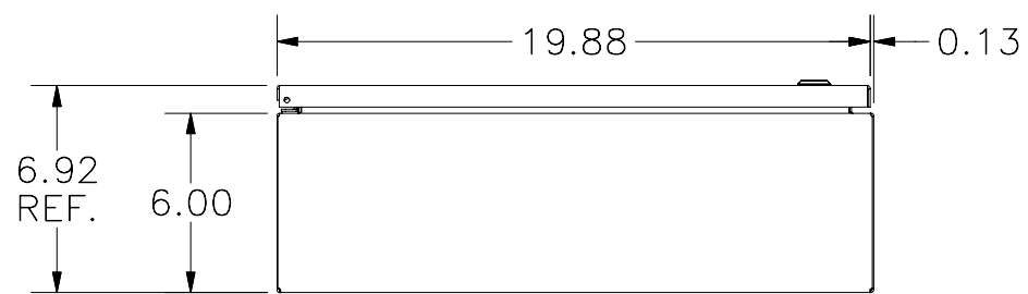
BOTTOM VIEW
