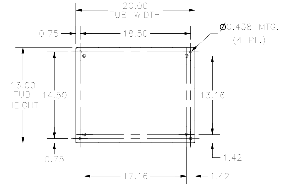
SECTION W-W (INSIDE BACK OF ENCLOSURE)
