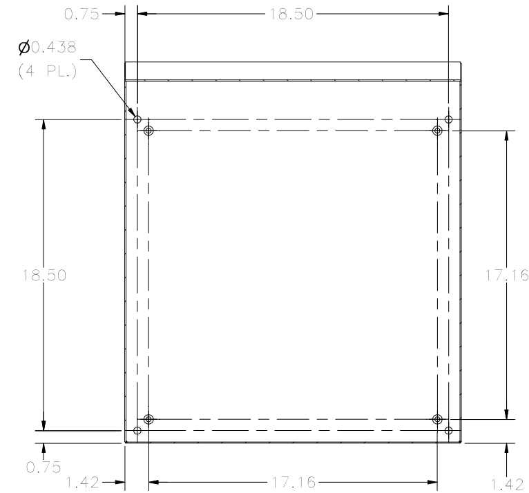
SECTION A-A VIEW (INSIDE BACK OF ENCL.)
