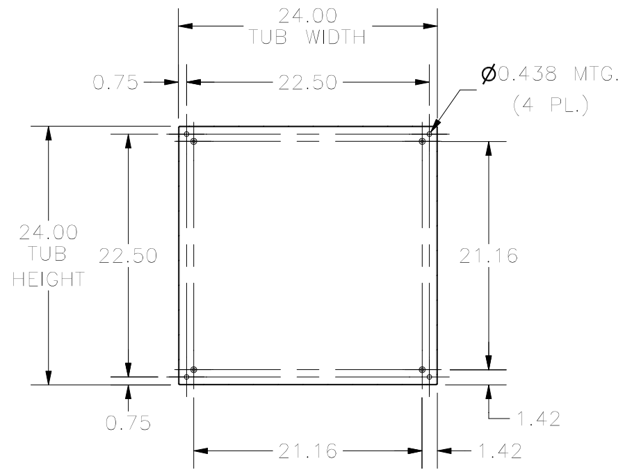
SECTION W-W (INSIDE BACK OF ENCLOSURE)
