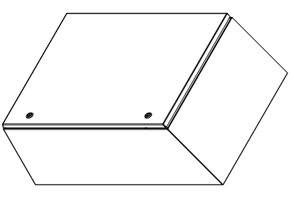
REF. VIEW (DOOR CLOSED)
