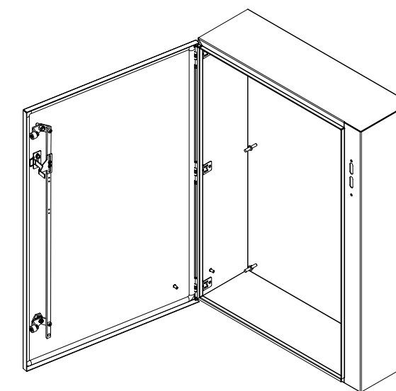
REF. VIEW (DOOR OPEN)
