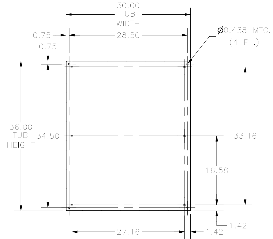
SECTION W-W (INSIDE BACK OF ENCLOSURE)
