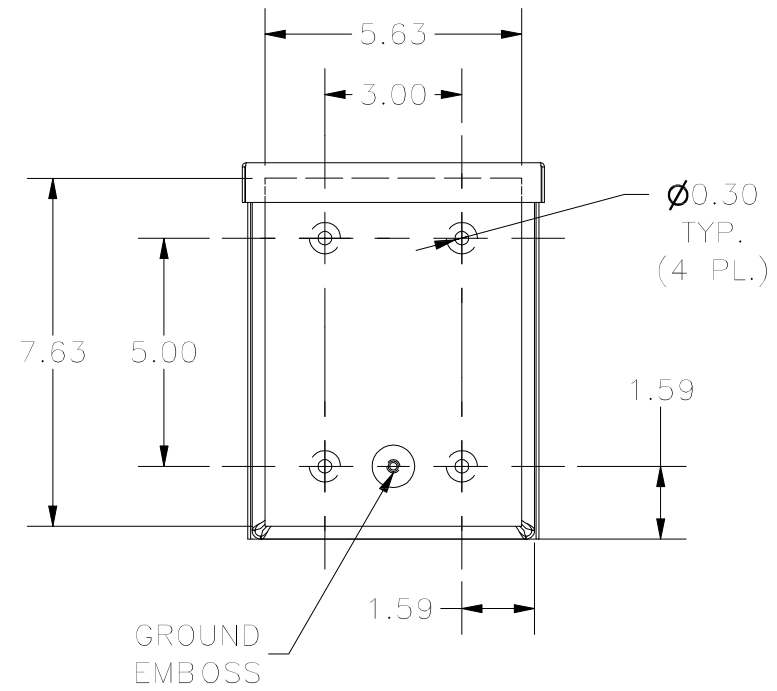
BACK VIEW
