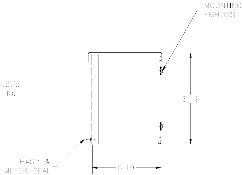
RIGHT VIEW
