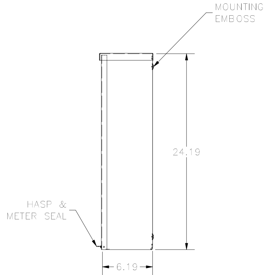
RIGHT VIEW
