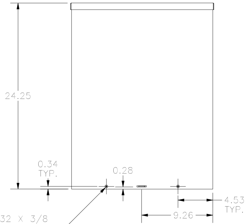
FRONT VIEW
