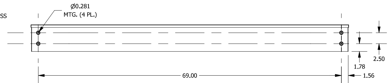
BACK VIEW
