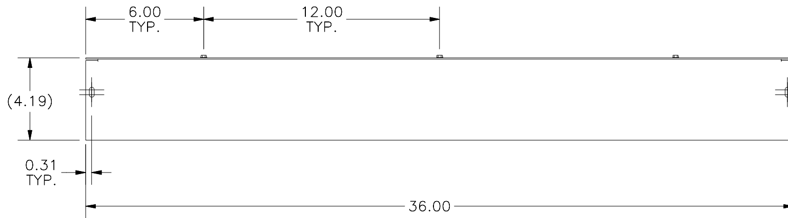
FRONT VIEW
