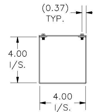
RIGHT VIEW
