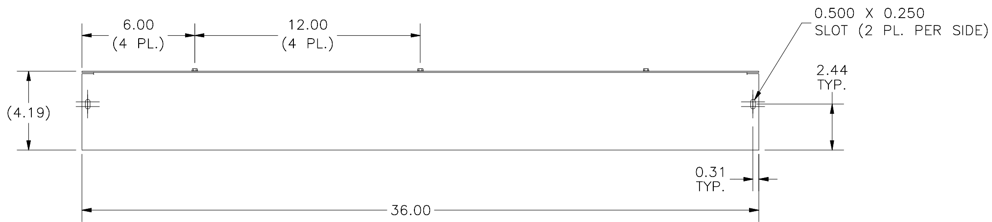
FRONT VIEW
