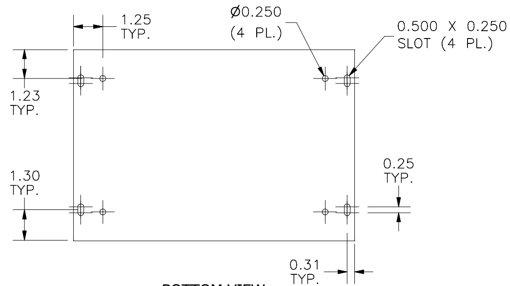
BOTTOM VIEW
