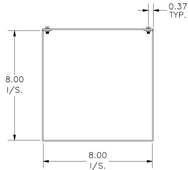
RIGHT VIEW
