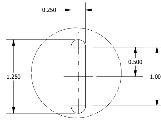
DETAIL A (22 PL.) (SLOT DETAIL)
