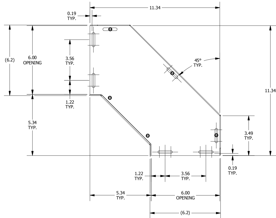
TOP VIEW
