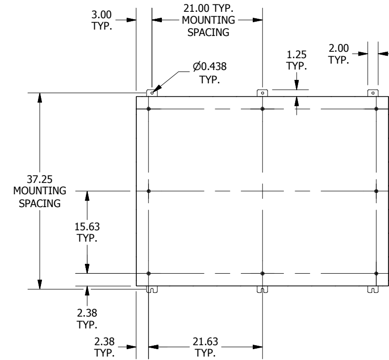
SECTION A-A (INSIDE BACK VIEW OF ENCL.)
