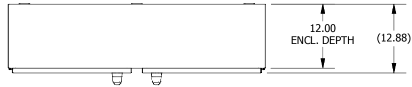
TOP VIEW
