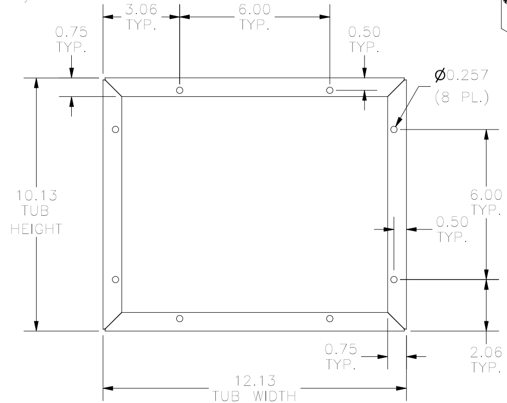
FRONT VIEW TUB
