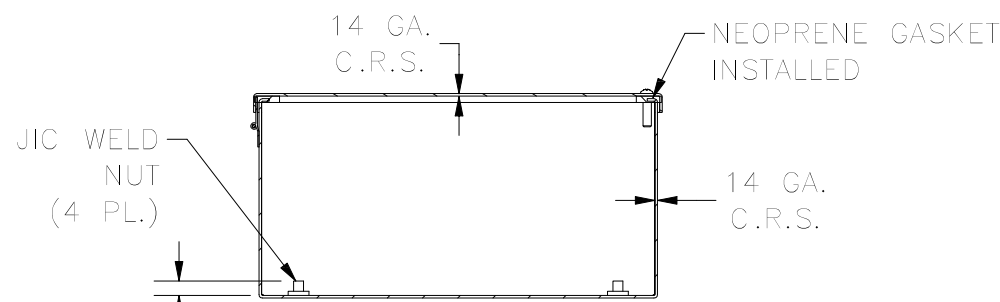
SECTION B-B VIEW (INSIDE TOP OF ENCL.)
