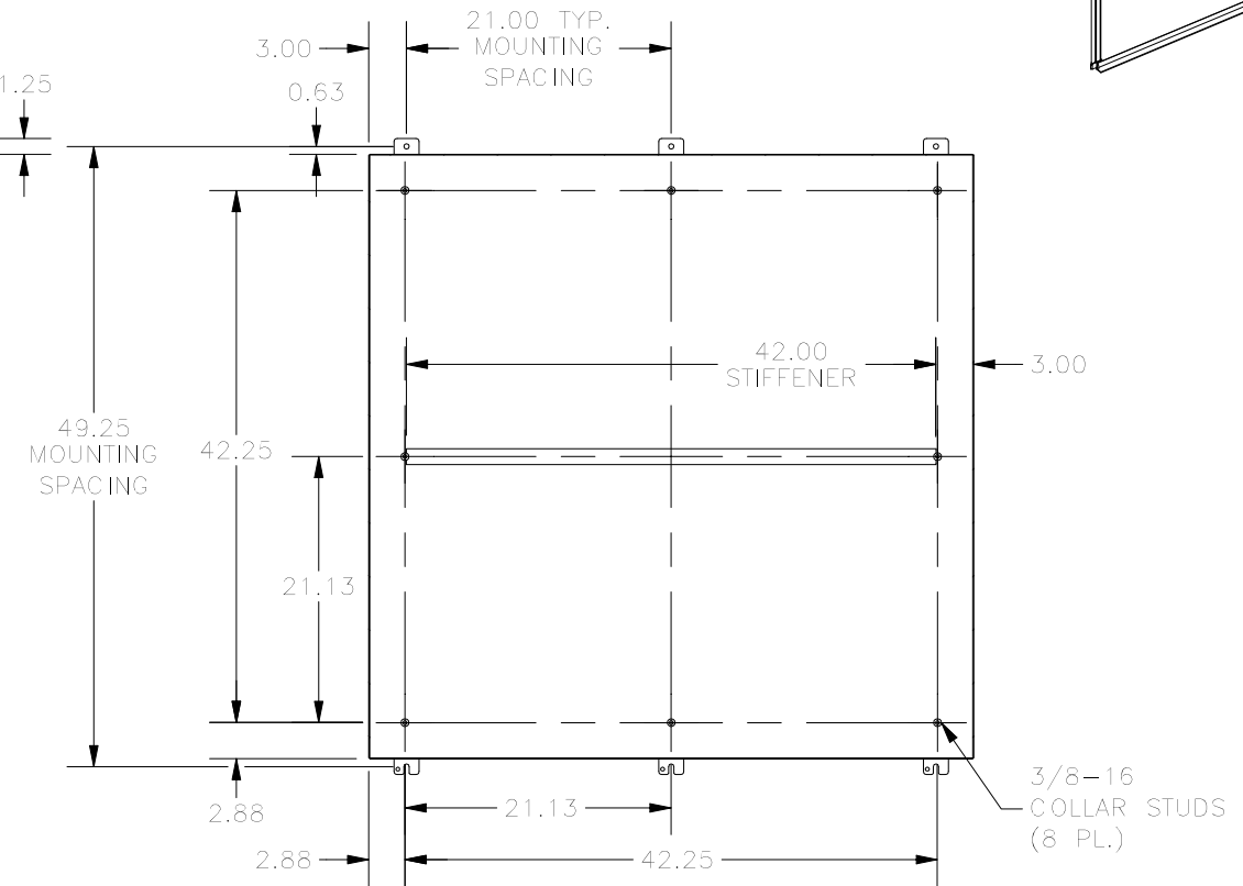
SECTION A-A (INSIDE BACK VIEW OF ENCL.)
