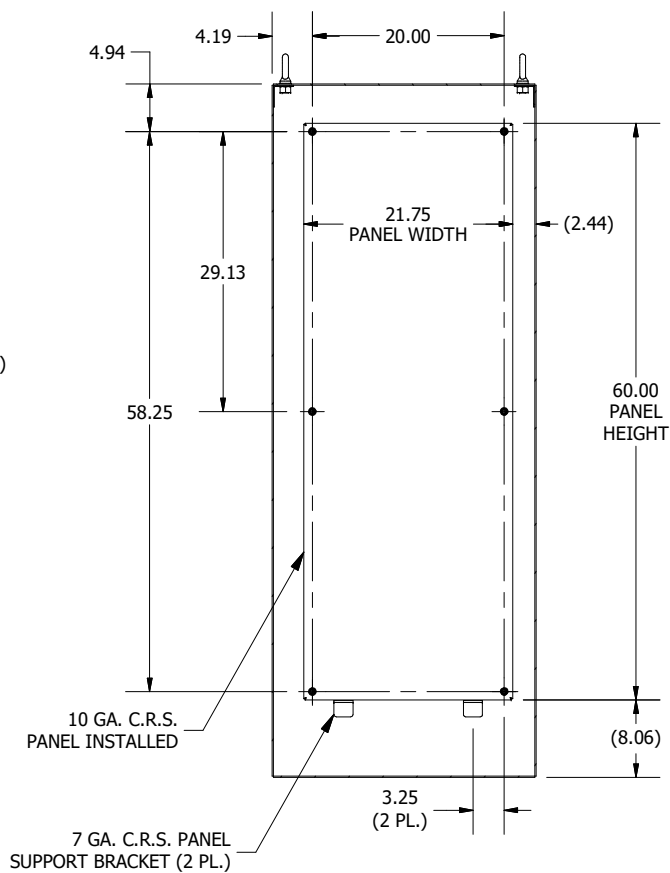
SECTION A-A (INSIDE BACK OF ENCL.)
