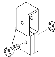
CLIP DETAIL
