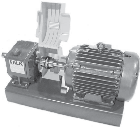
Concentric Drive & High-Speed Flexible Coupling with Type MCG Guard
