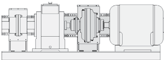
Type CFCG and SCG with Fluid & Gear Coupling
