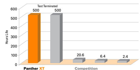
PANTHER XT Belt Life Comparison
