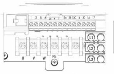
Three Phase (3/PE)
