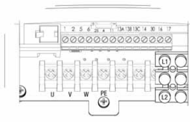
Single Phase (2/PE)
