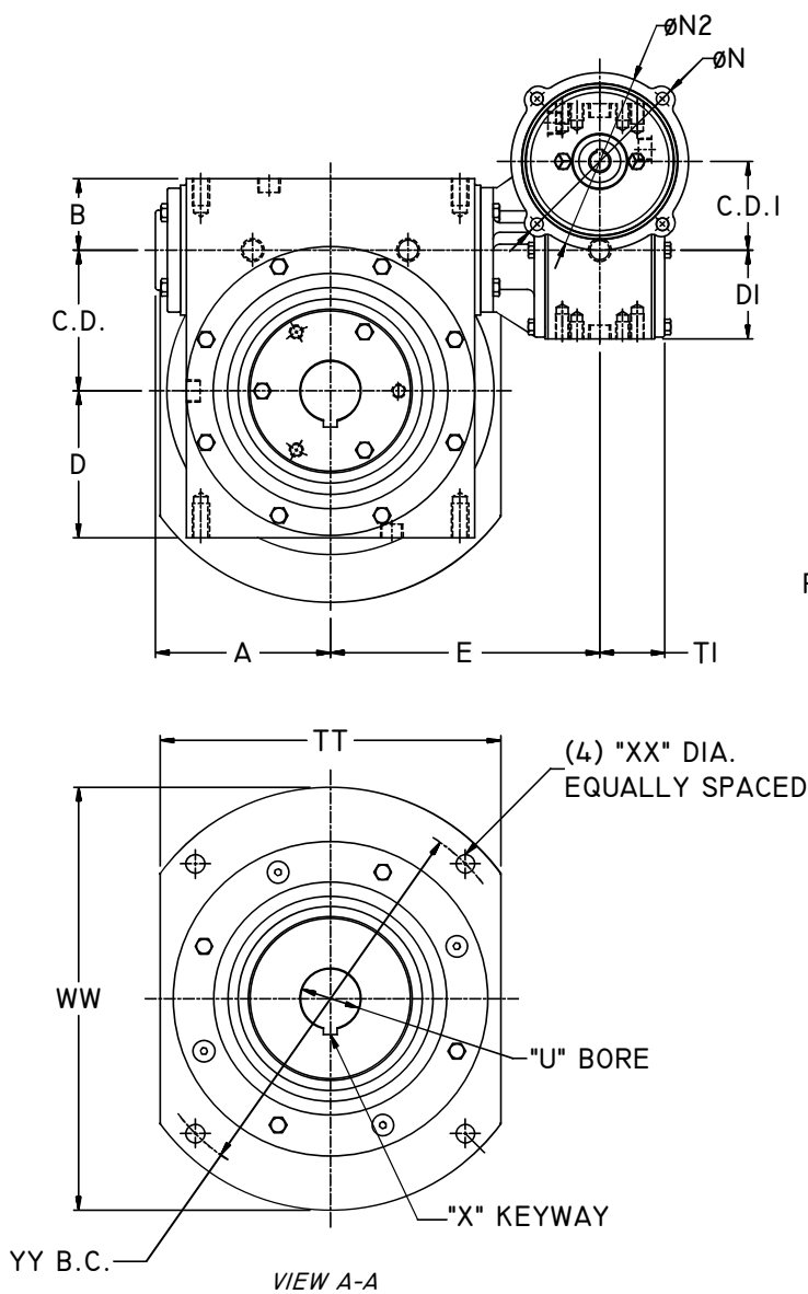
Detail for Models 1506, 3006, 4206 F-Flange
