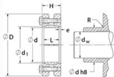
Shrink Disc
