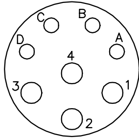
8 PIN THREADED CONNECTOR (CRIMP STYLE) (INSERTION SIDE)
