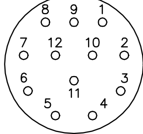
12 PIN THREADED CONNECTOR (CRIMP STYLE) (INSERTION SIDE)
