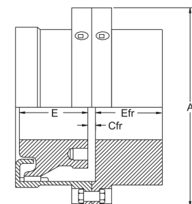
Flex-Rigid Coupling
