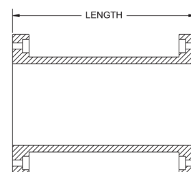
Spacer Spacer Length + C = Hub Separation
