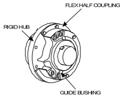
FLOATING SHAFT IDENTICAL TO FLEX RIGID BUT WITH GUIDE BUSHINGS
