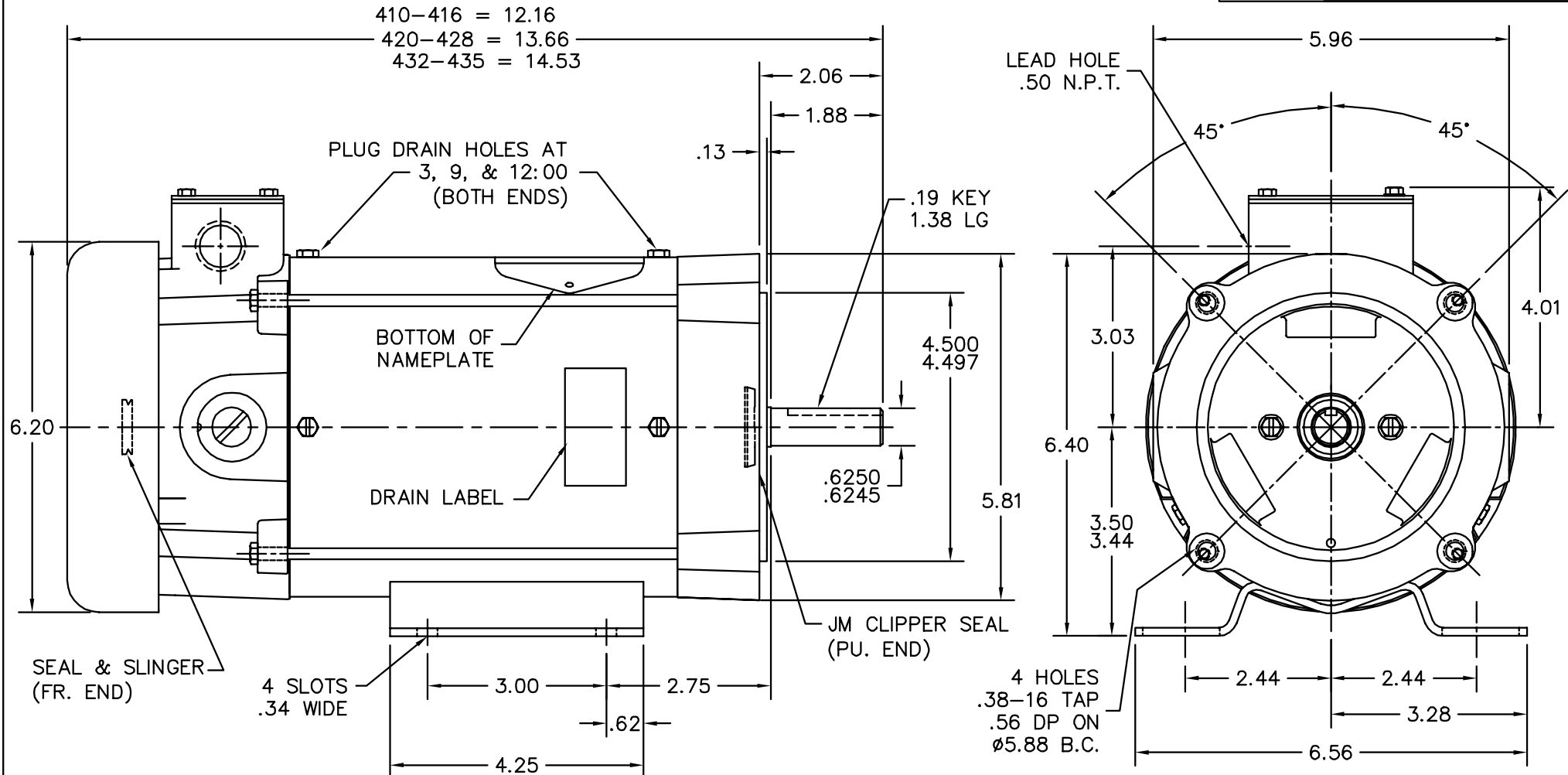
DETAILS OF FR END
