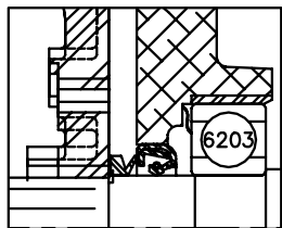
DETAILS OF FR END
