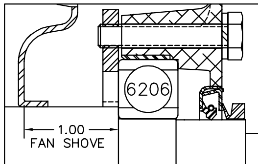
PULLEY END DETAIL
