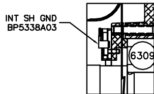
PUL BRG RETAINER DETAIL
