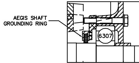
PULLEY END DETAIL
