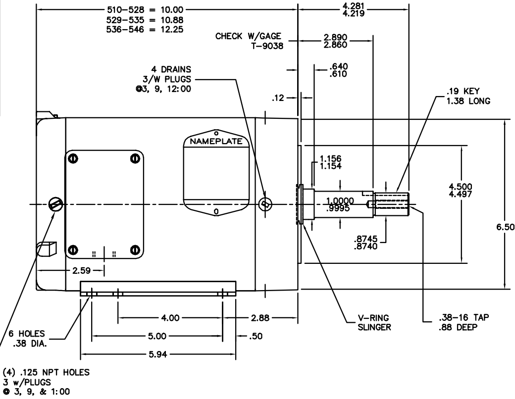
PULLEY END DETAIL
