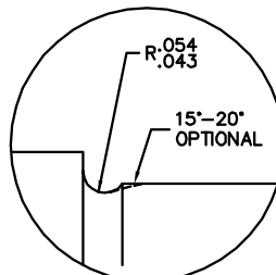
UNDERCUT DETAIL
