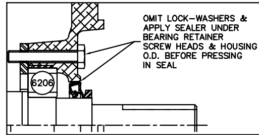
PULLEY END DETAIL
